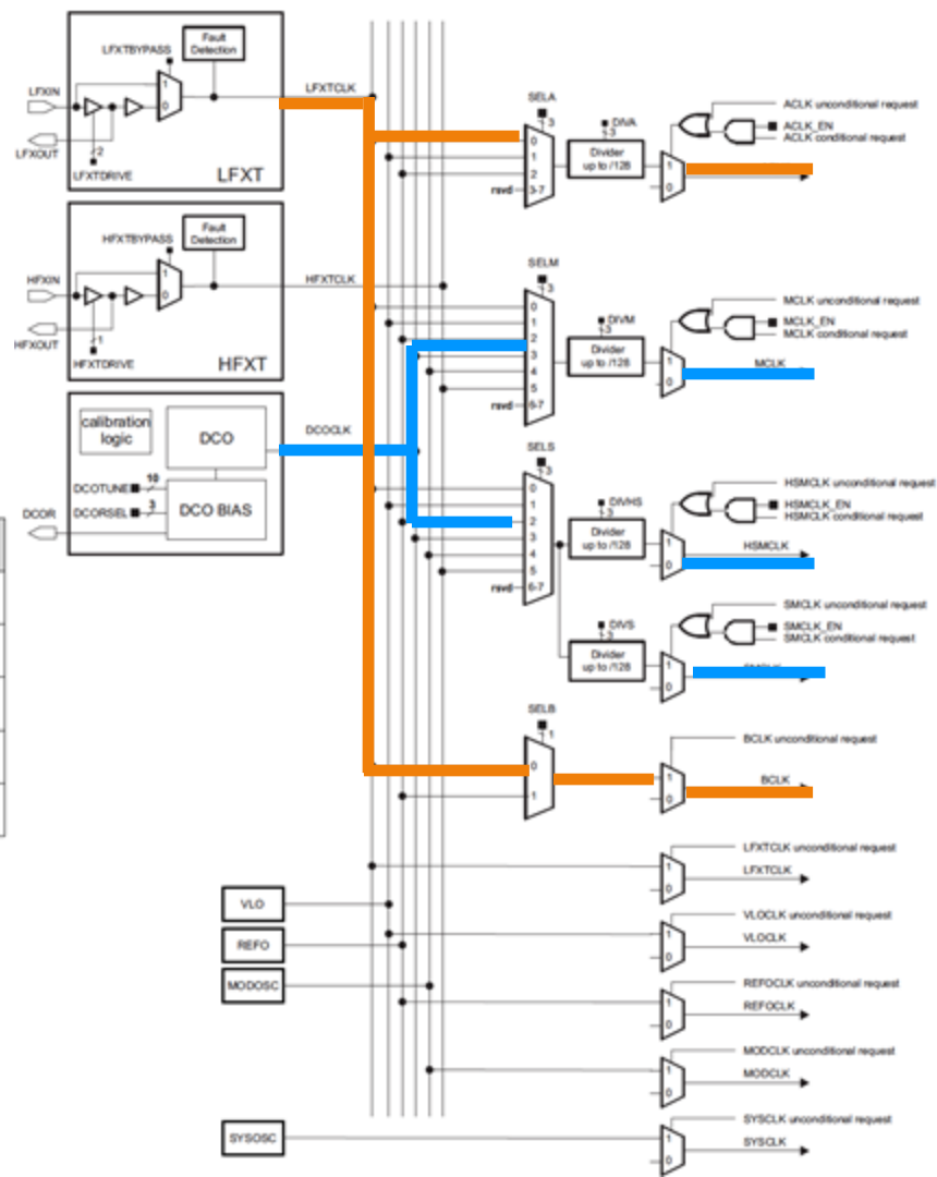
Clock Default Clock Source Default Clock Frequency Description MCLK DCO 3 MHz Master Clock Sources CPU and peripherals HSMCLK DCO 3 MHz Subsystem Master Clock Sources peripherals SMCLK DCO 3 MHz Low-speed subsystem master clock Sources peripherals ACLK LFXT (or REFO if no crystal present) 32.768 kHz Auxiliary clock Sources peripherals BCLK LFXT (or REFO if no crystal present) 32.768 kHz Low-speed backup domain clock Sources LPM peripherals
