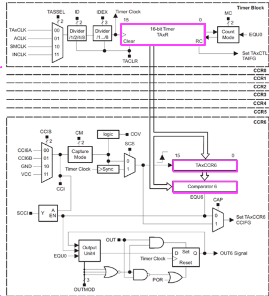
Figure 17-1. Timer_A Block Diagram
