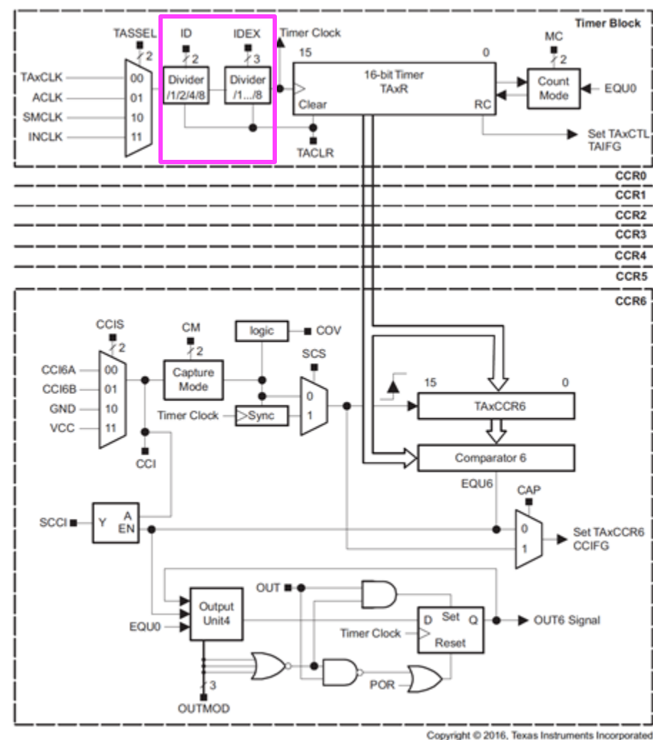
Figure 17-1. Timer_A Block Diagram
